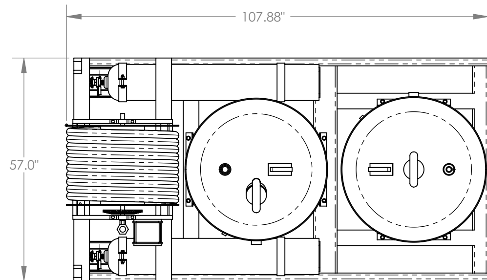
TOP VIEW
